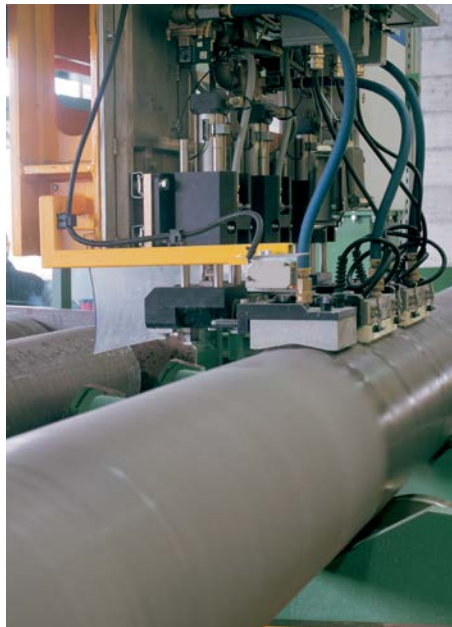
Automatic ultrasonic control system for the entire length of the billet according to class "A" of SAE AMS-STD-2154 regulation
